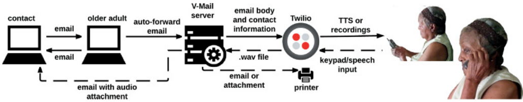
Fig. 1. Depicts how messages are received (solid line) and sent (dashed line) by older adults using V-Mail. Older adults interact through keypad input on their landline or cellular telephones. They can send a message by speaking directly into the phone, which transmits to the recipients e-mail account.
